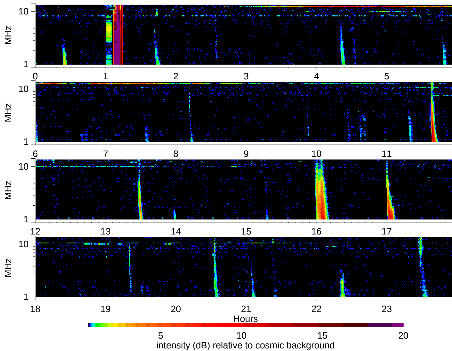
Wind Waves RAD2 receiver: 2006/11/22
