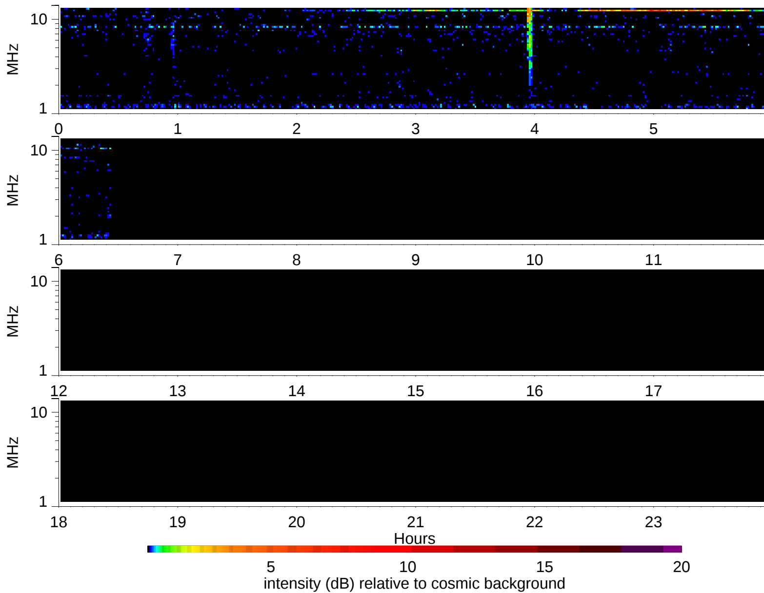
Wind Waves RAD2 receiver: 2006/11/23
