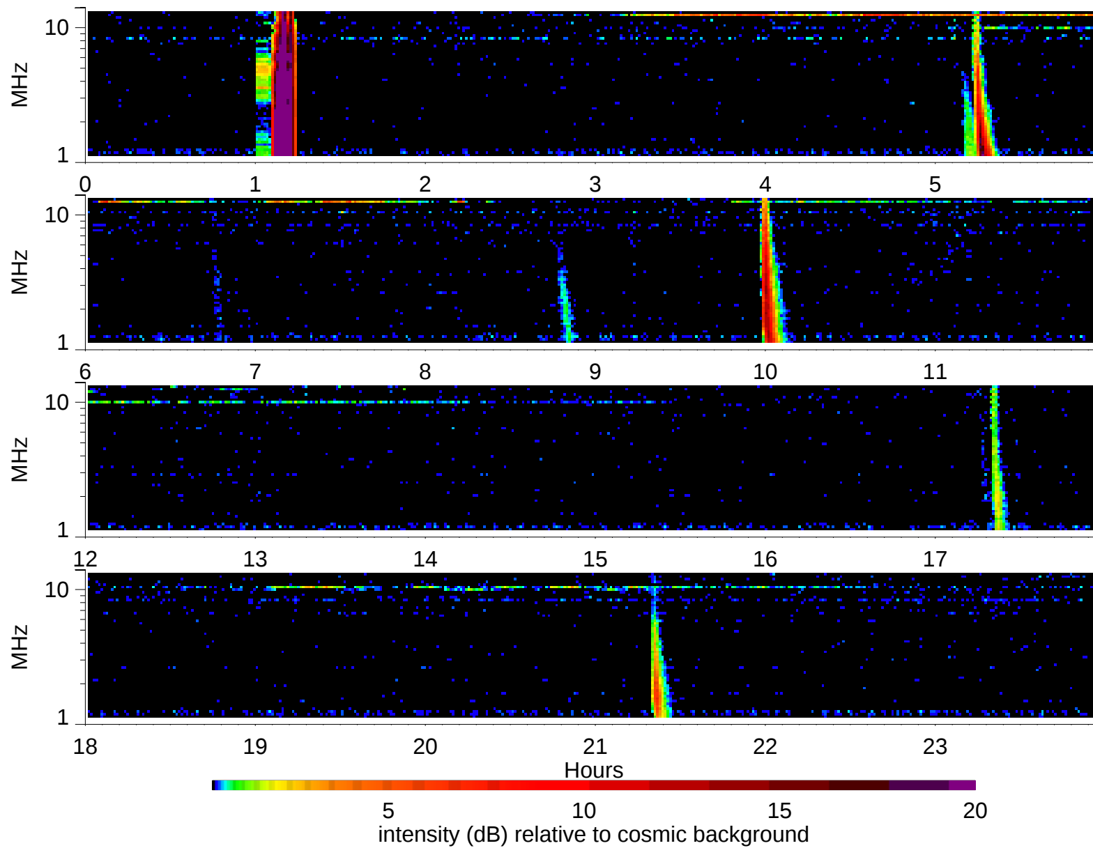
Wind Waves RAD2 receiver: 2006/12/2
