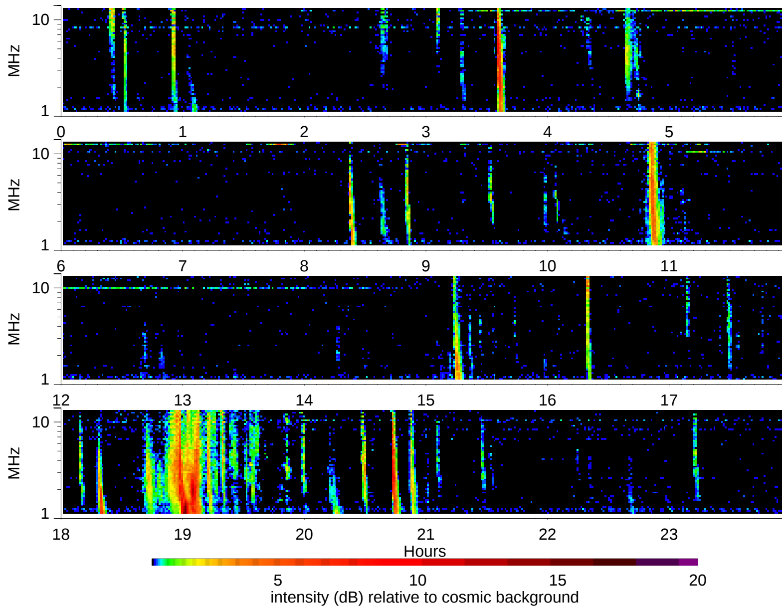
Wind Waves RAD2 receiver: 2006/12/7
