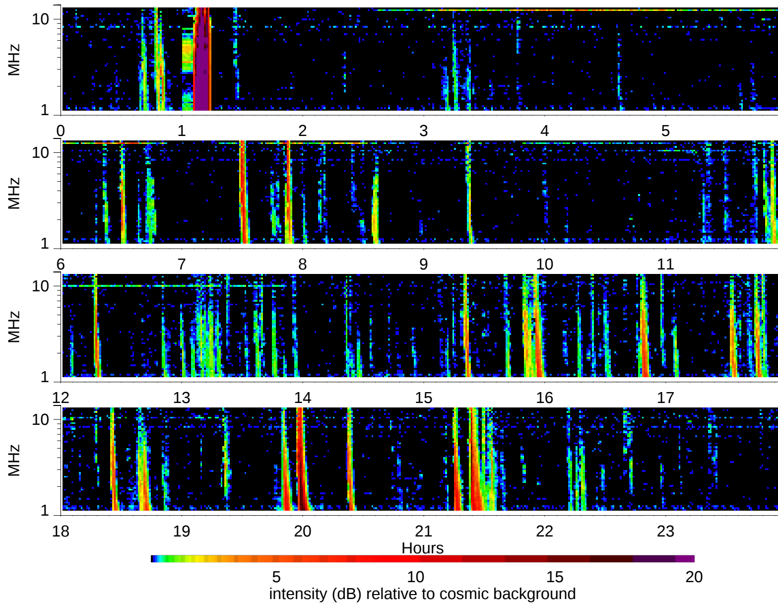
Wind Waves RAD2 receiver: 2006/12/10
