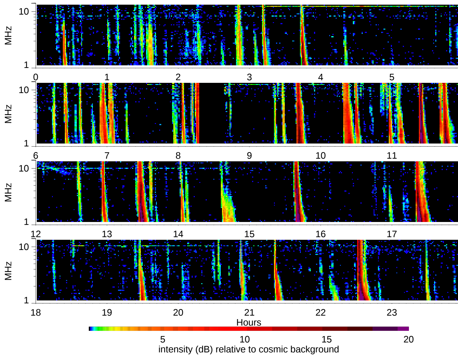
Wind Waves RAD2 receiver: 2006/12/11
