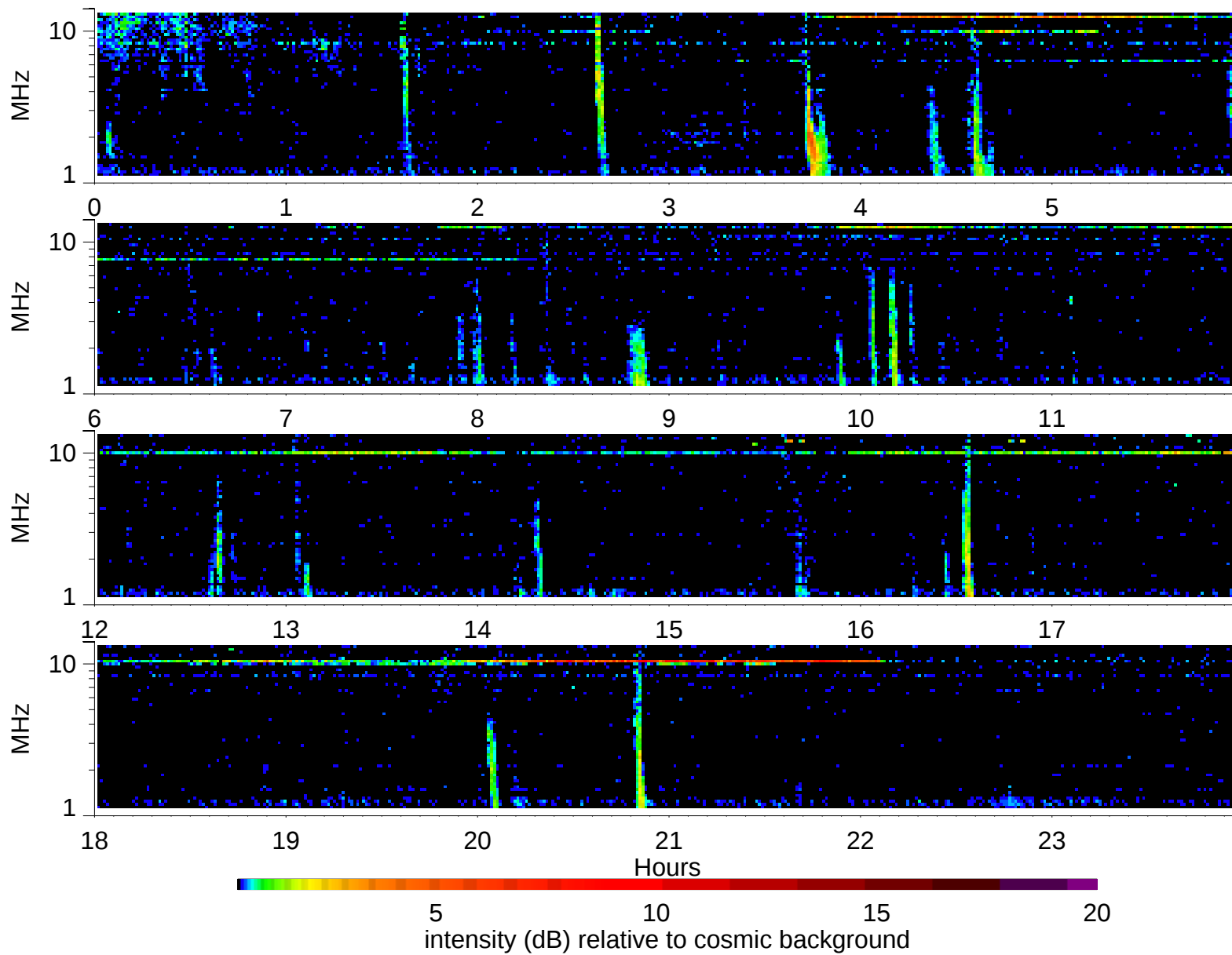
Wind Waves RAD2 receiver: 2006/12/15
