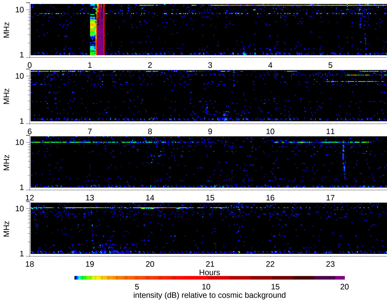
Wind Waves RAD2 receiver: 2006/12/16
