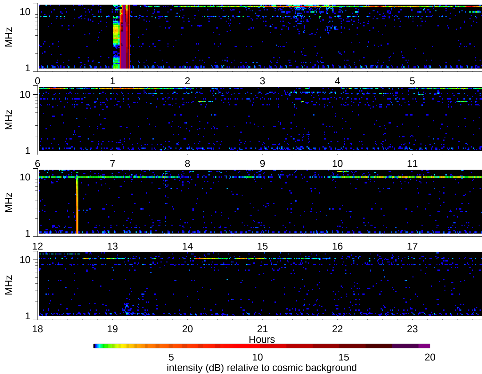
Wind Waves RAD2 receiver: 2006/12/20
