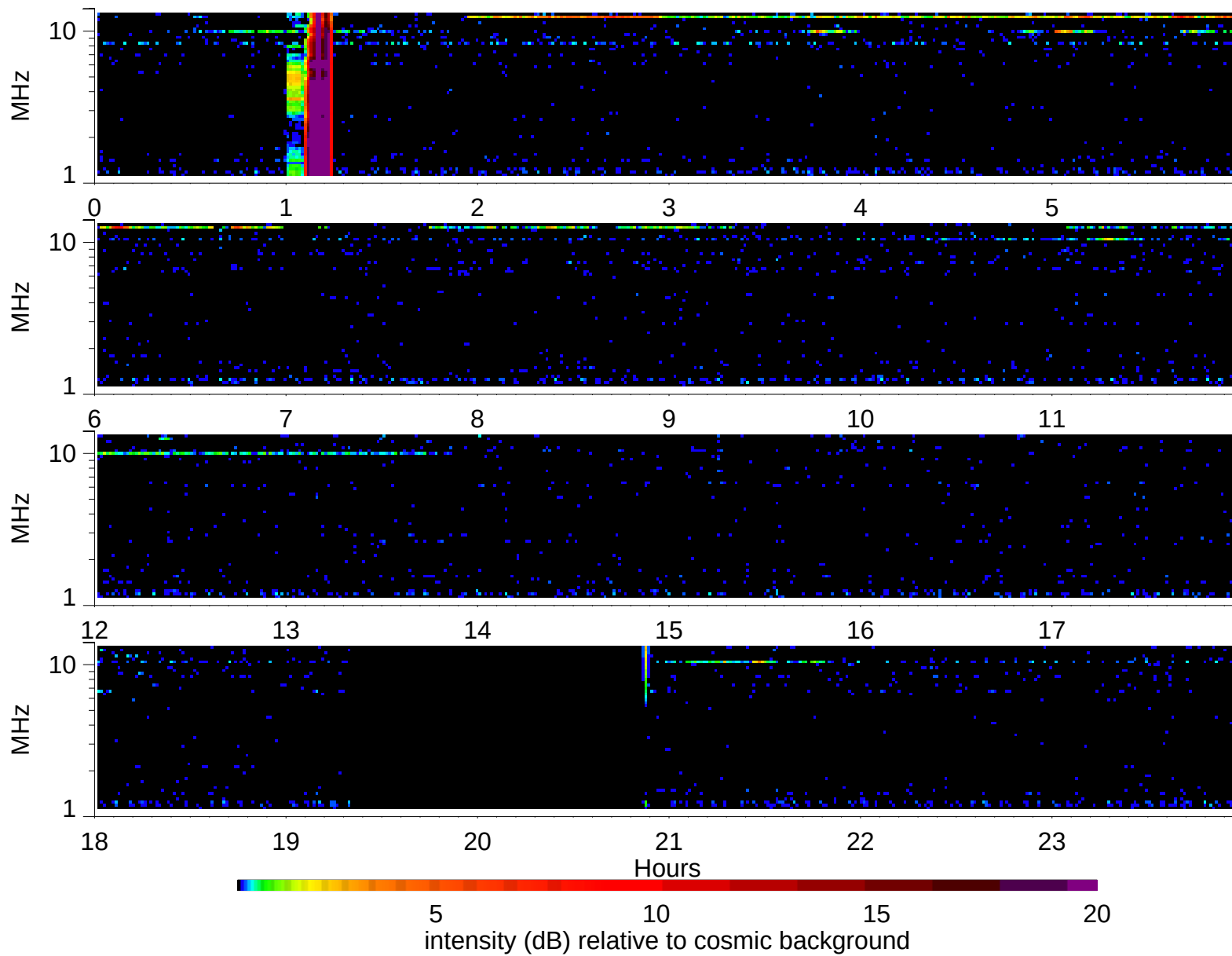
Wind Waves RAD2 receiver: 2006/12/24
