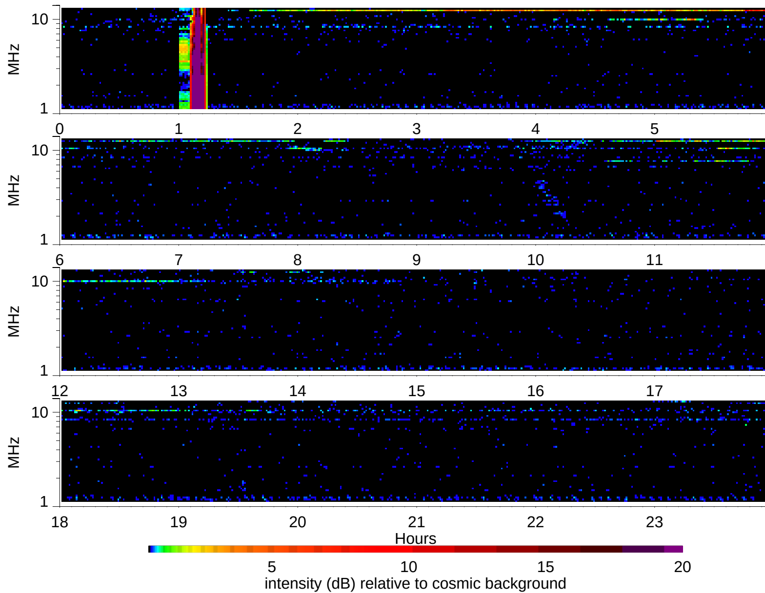
Wind Waves RAD2 receiver: 2006/12/26
