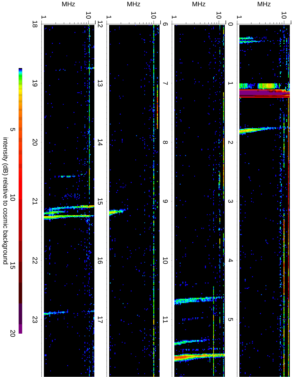
Wind Waves RAD2 receiver: 2007/01/14
