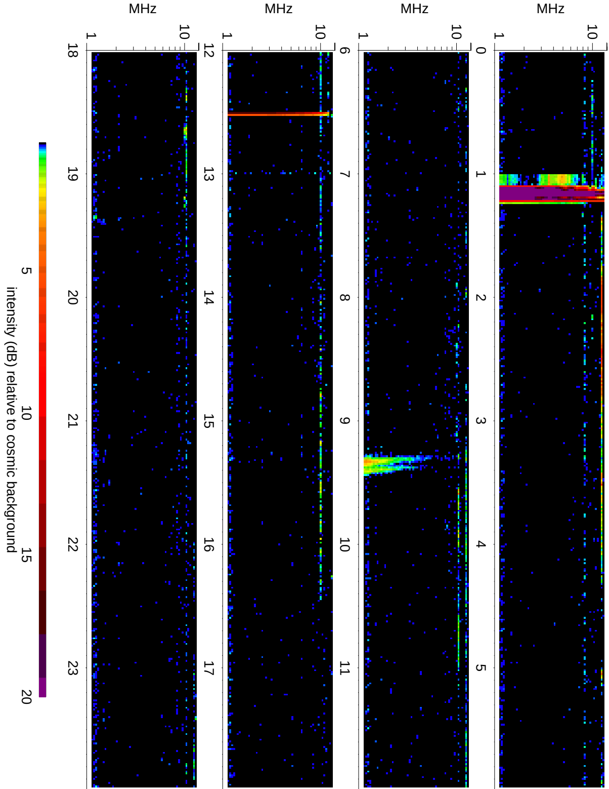
Wind Waves RAD2 receiver: 2007/01/18
