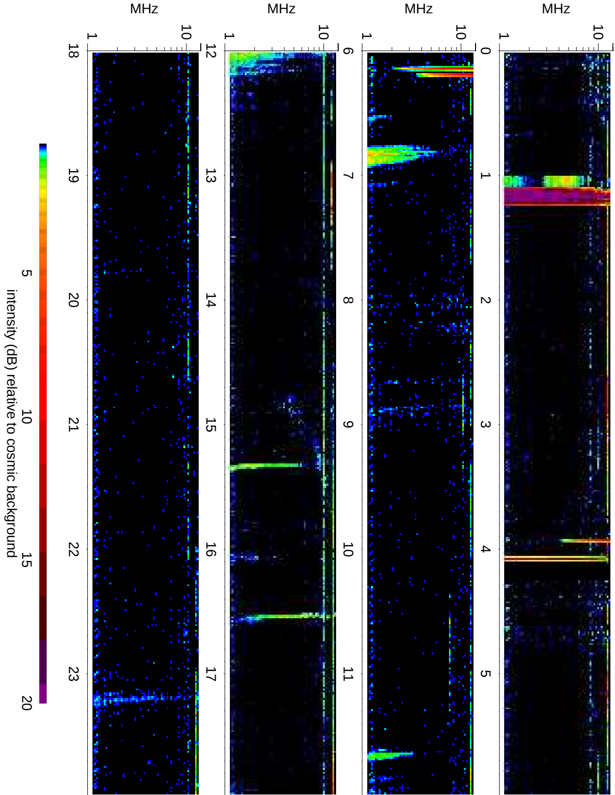
Wind Waves RAD2 receiver: 2007/02/01
