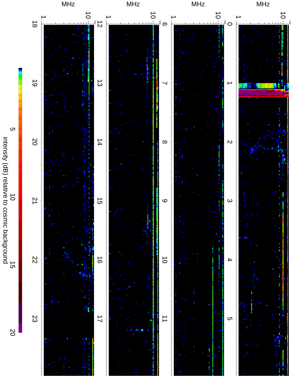
Wind Waves RAD2 receiver: 2007/02/21
