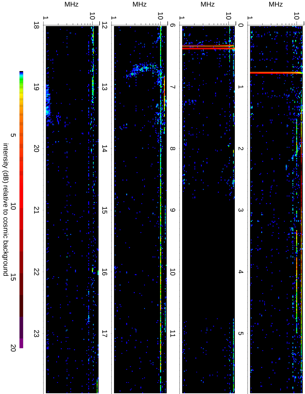
Wind Waves RAD2 receiver: 2007/03/12
