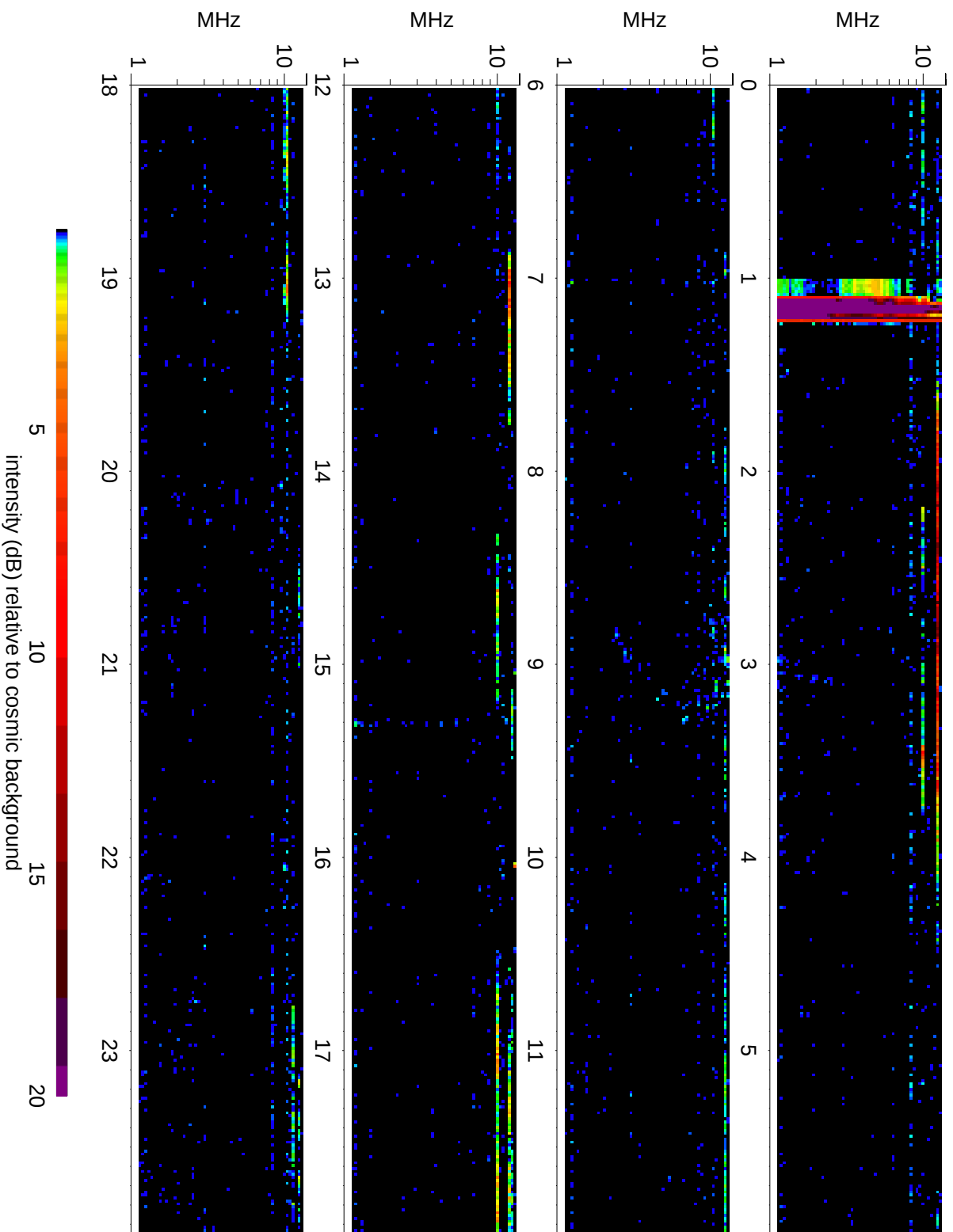
Wind Waves RAD2 receiver: 2007/03/13
