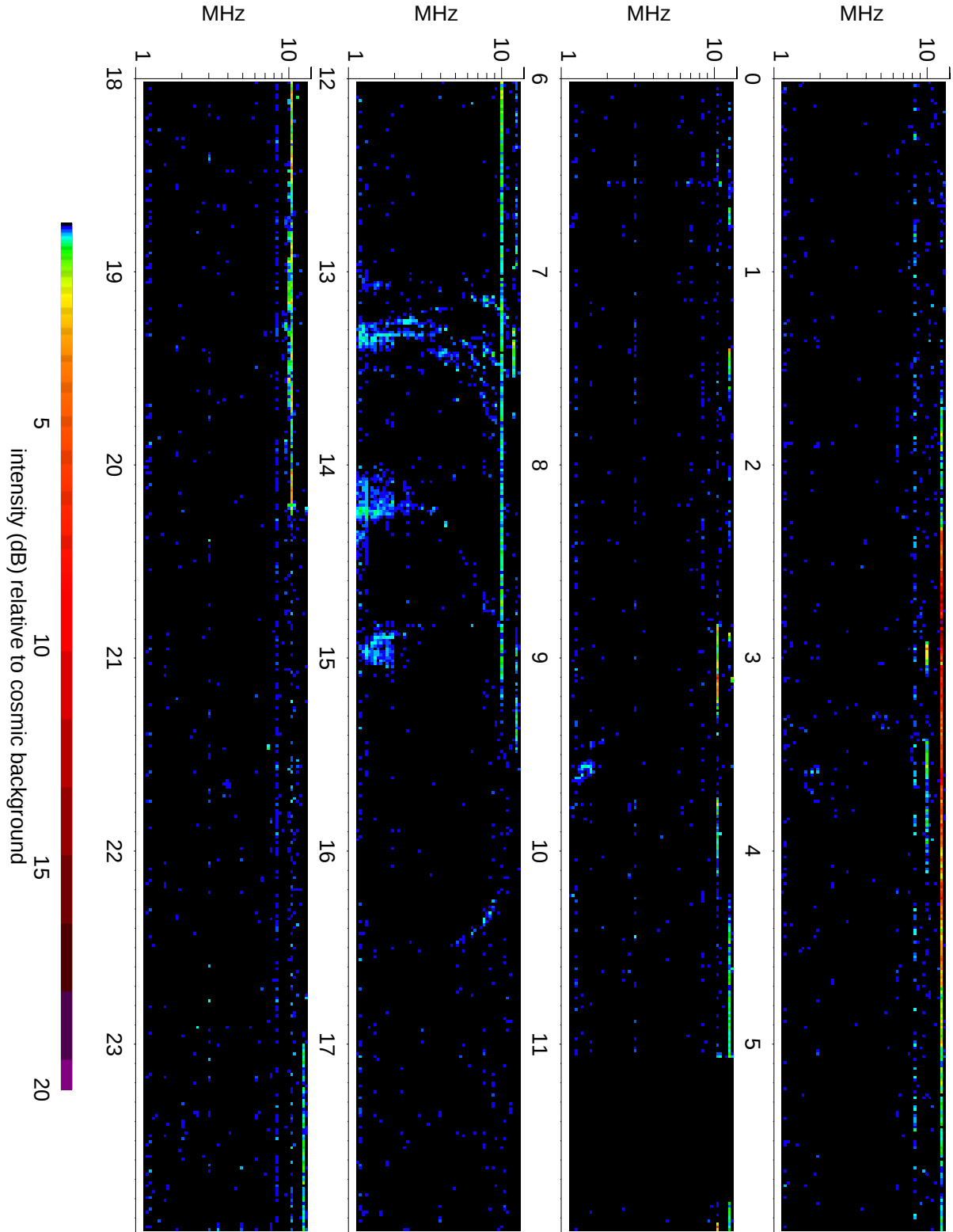
Wind Waves RAD2 receiver: 2007/03/16
