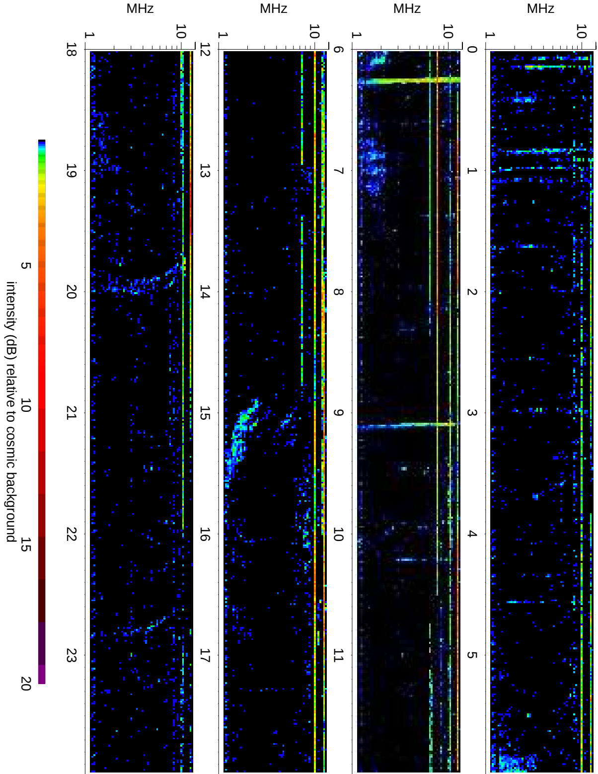
Wind Waves RAD2 receiver: 2007/05/11
