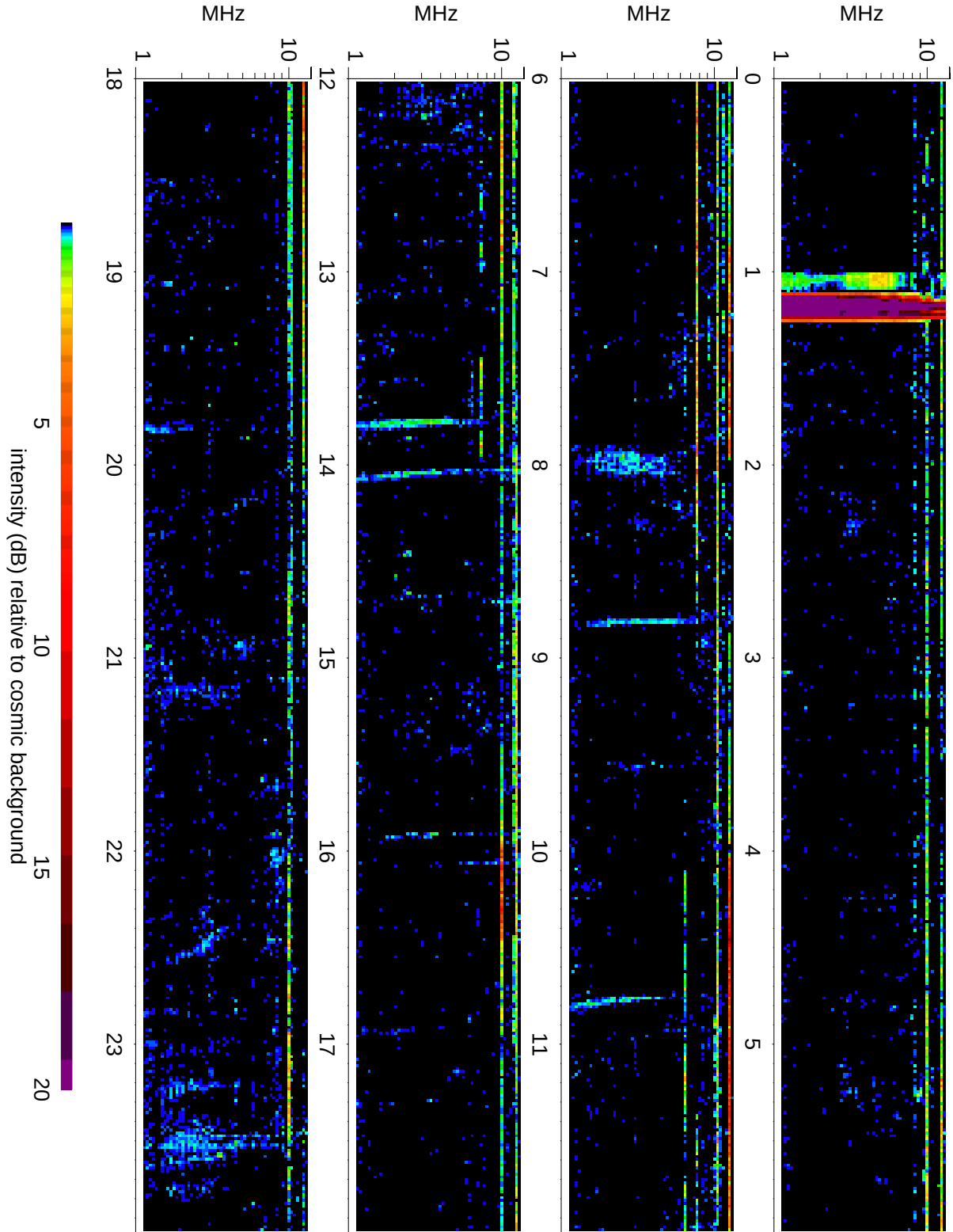
Wind Waves RAD2 receiver: 2007/06/07
