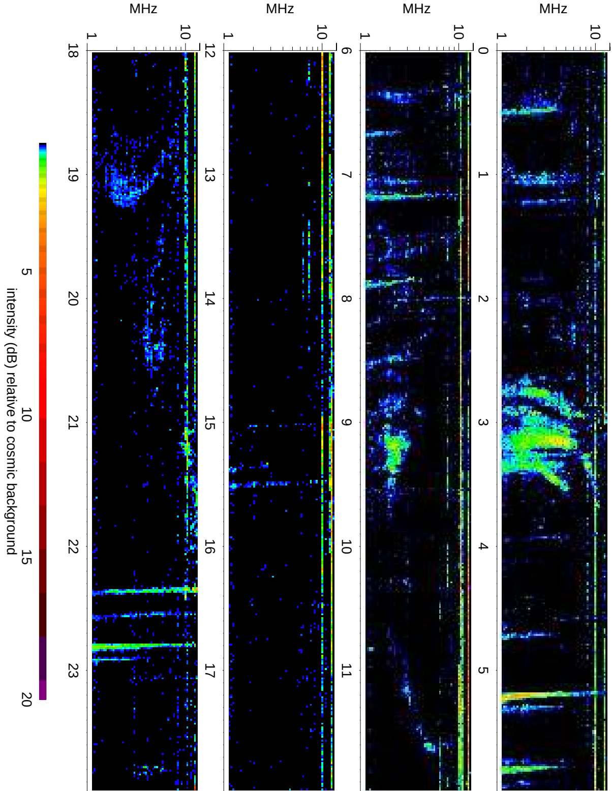
Wind Waves RAD2 receiver: 2007/06/08
