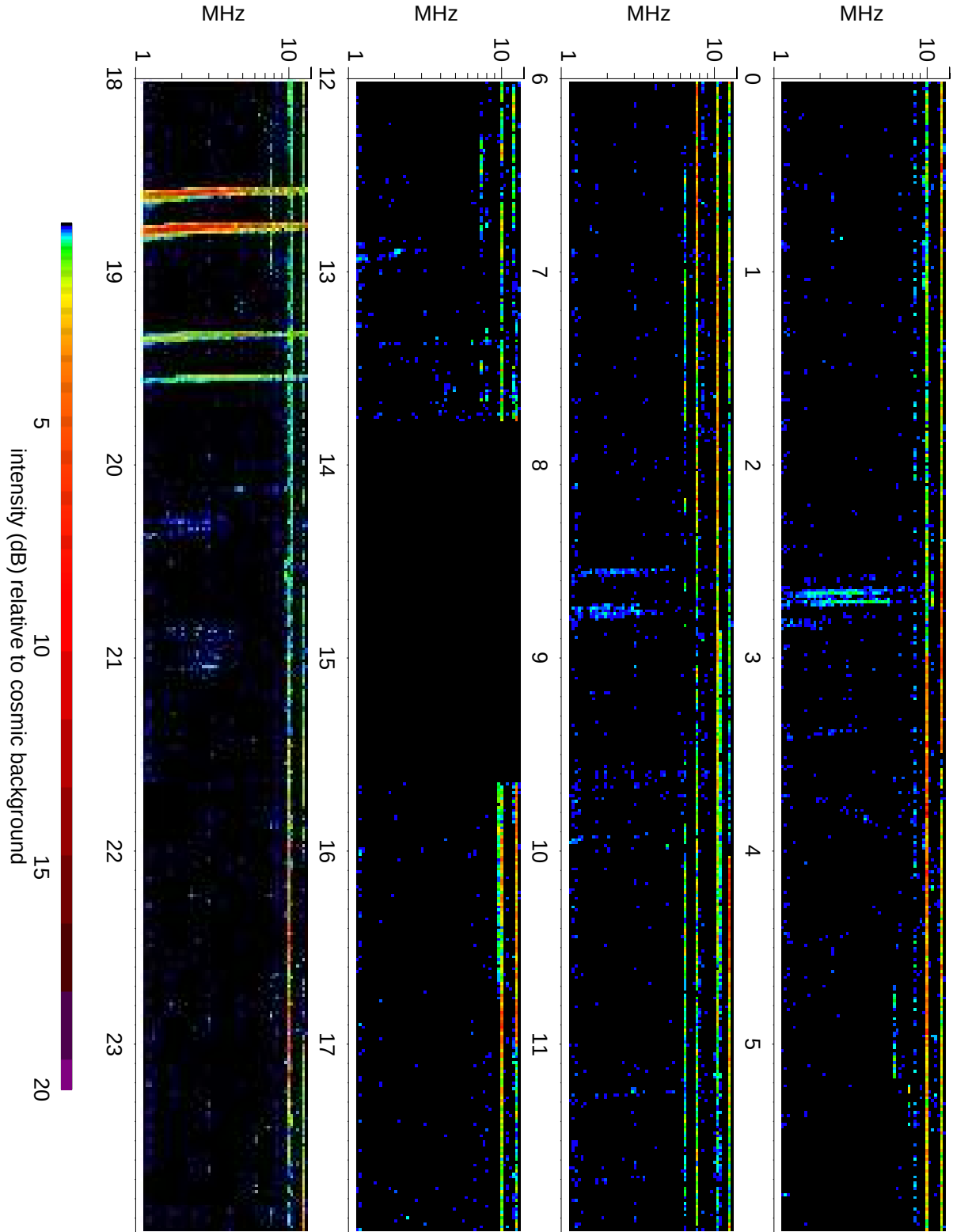
Wind Waves RAD2 receiver: 2007/07/04
