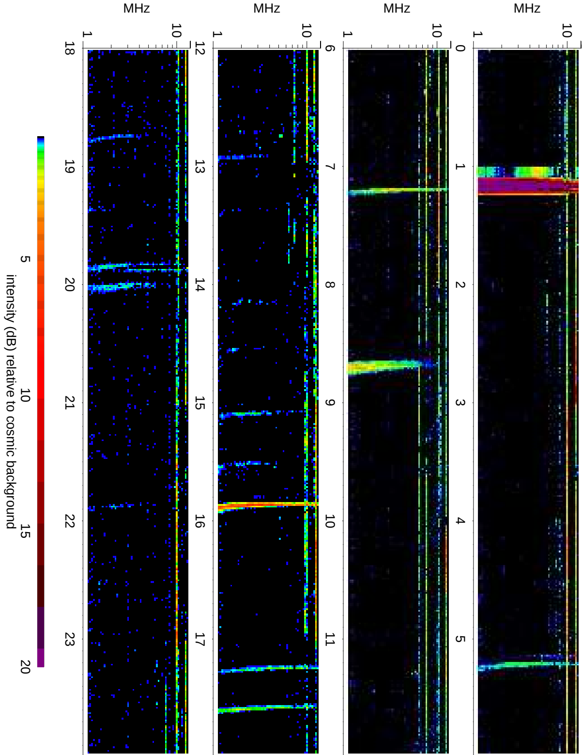
Wind Waves RAD2 receiver: 2007/07/05
