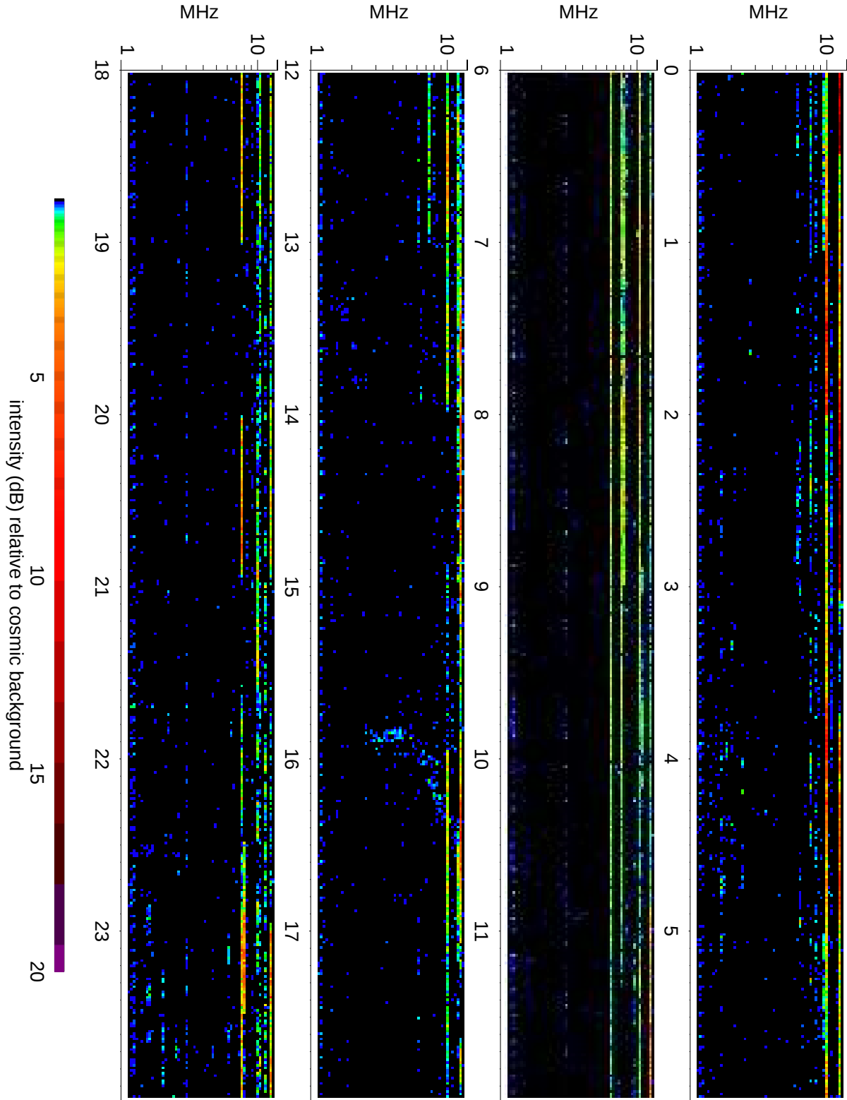
Wind Waves RAD2 receiver: 2007/08/11
