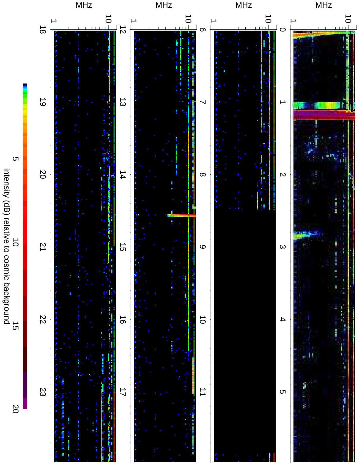
Wind Waves RAD2 receiver: 2007/08/24
