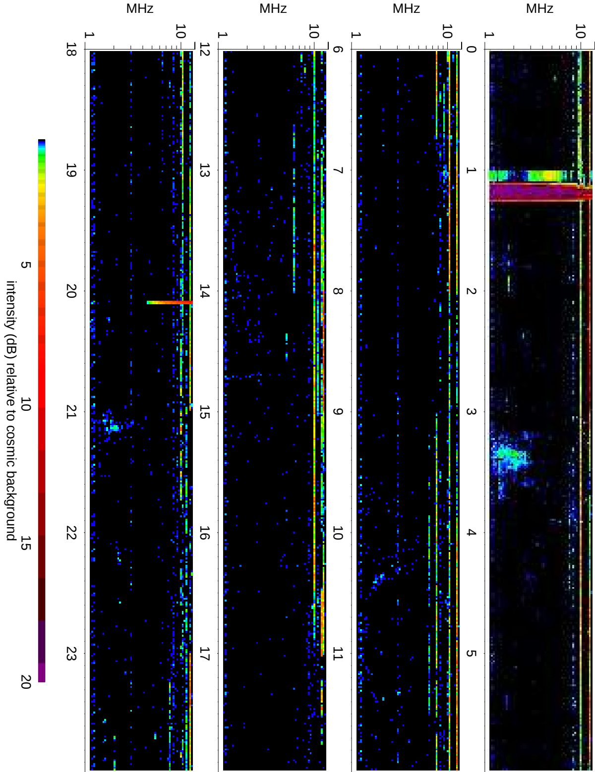
Wind Waves RAD2 receiver: 2007/08/30
