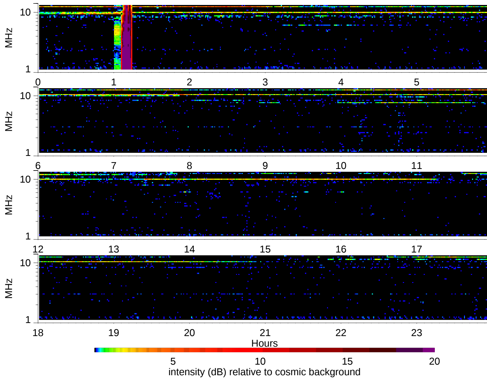
Wind Waves RAD2 receiver: 2007/9/11
