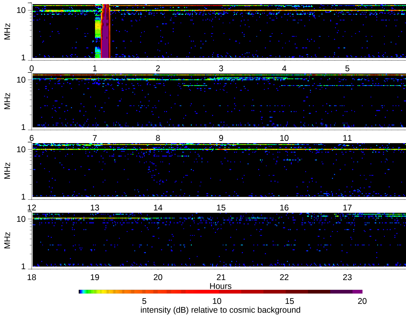
Wind Waves RAD2 receiver: 2007/9/19
