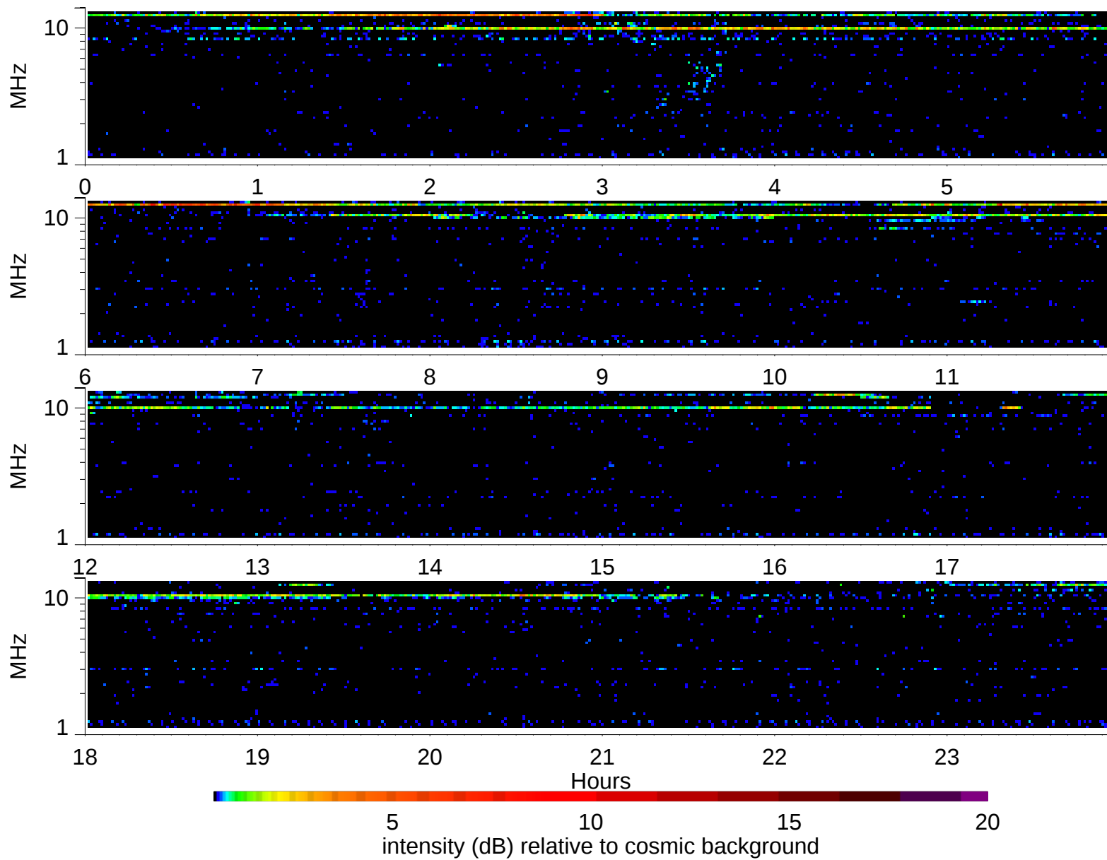
Wind Waves RAD2 receiver: 2007/9/22
