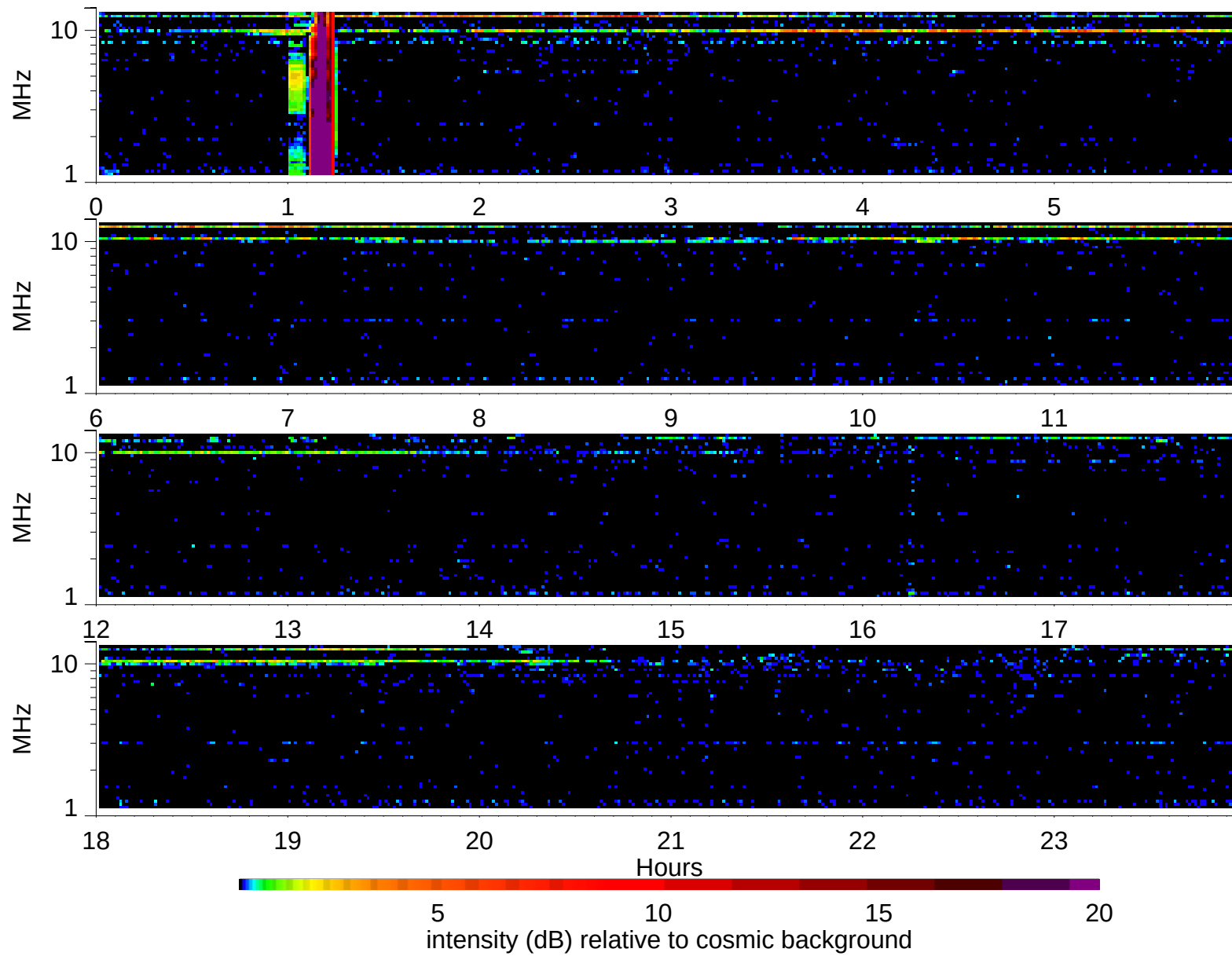
Wind Waves RAD2 receiver: 2007/9/23
