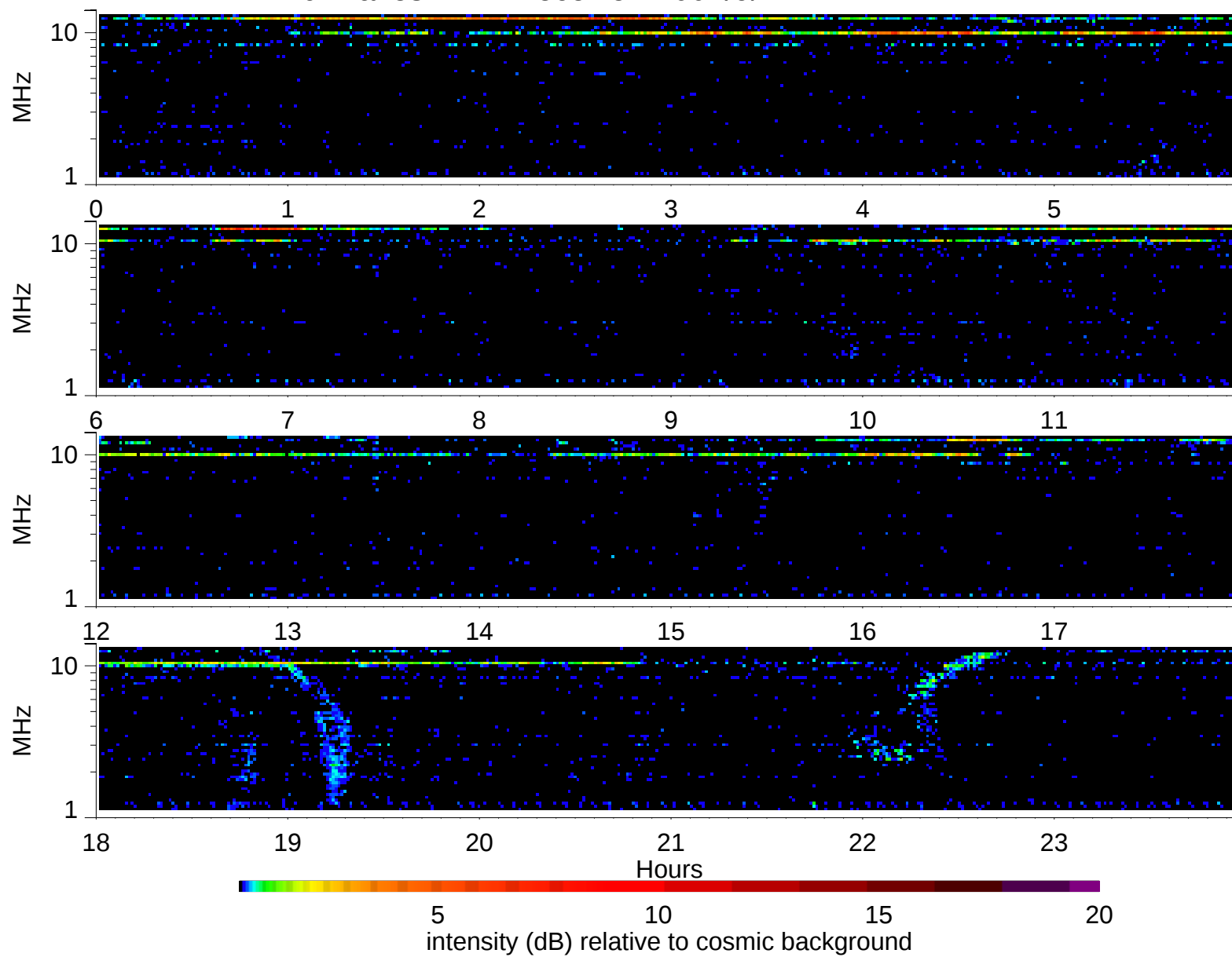
Wind Waves RAD2 receiver: 2007/9/24
