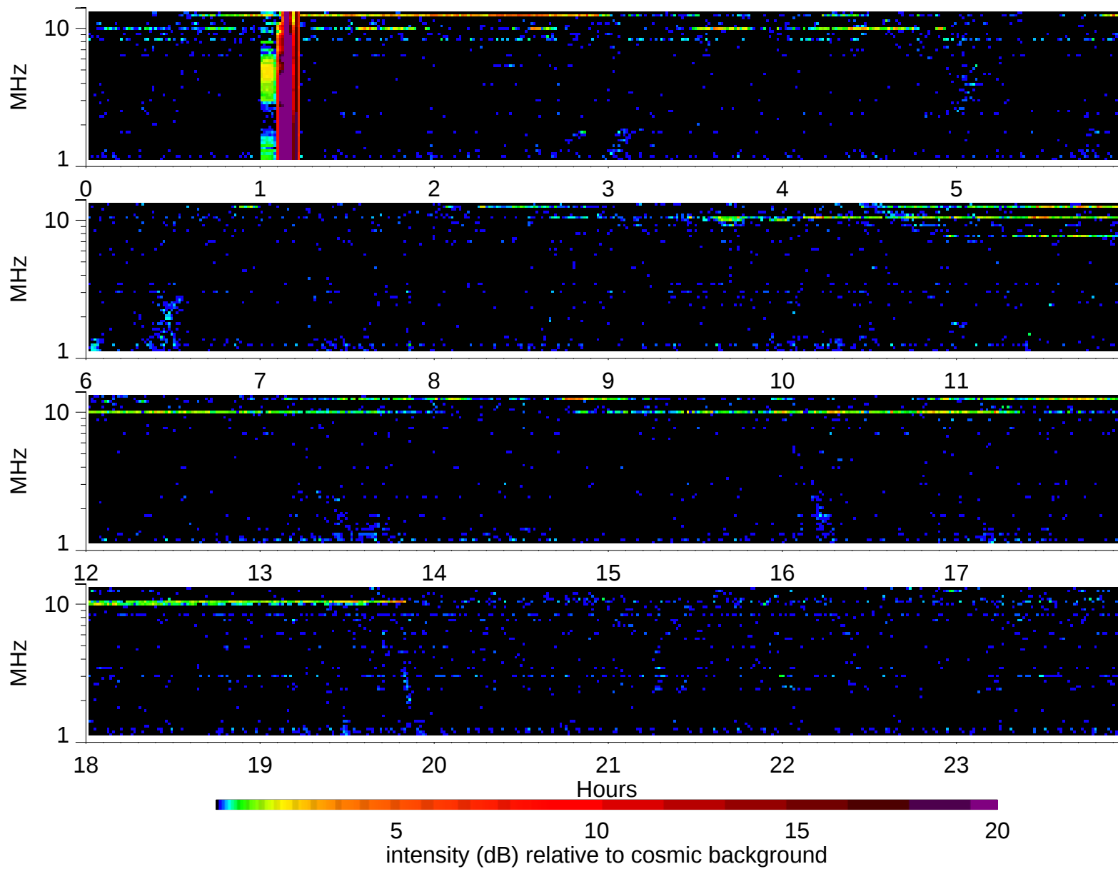
Wind Waves RAD2 receiver: 2007/9/29
