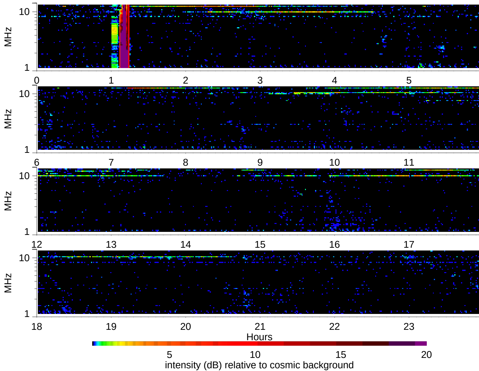
Wind Waves RAD2 receiver: 2007/10/1
