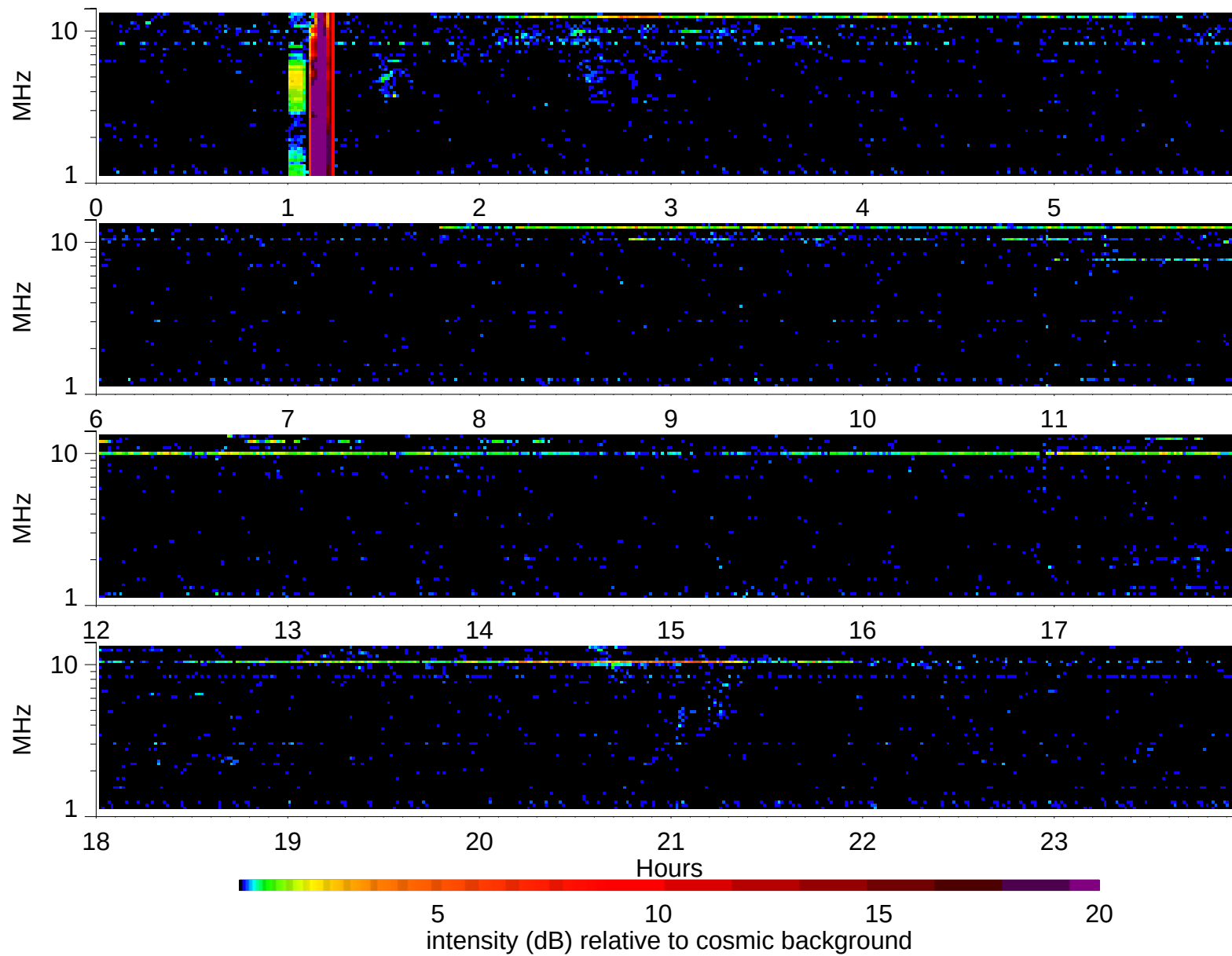
Wind Waves RAD2 receiver: 2007/10/9
