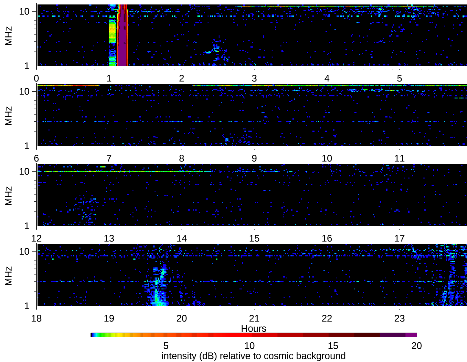
Wind Waves RAD2 receiver: 2007/10/15
