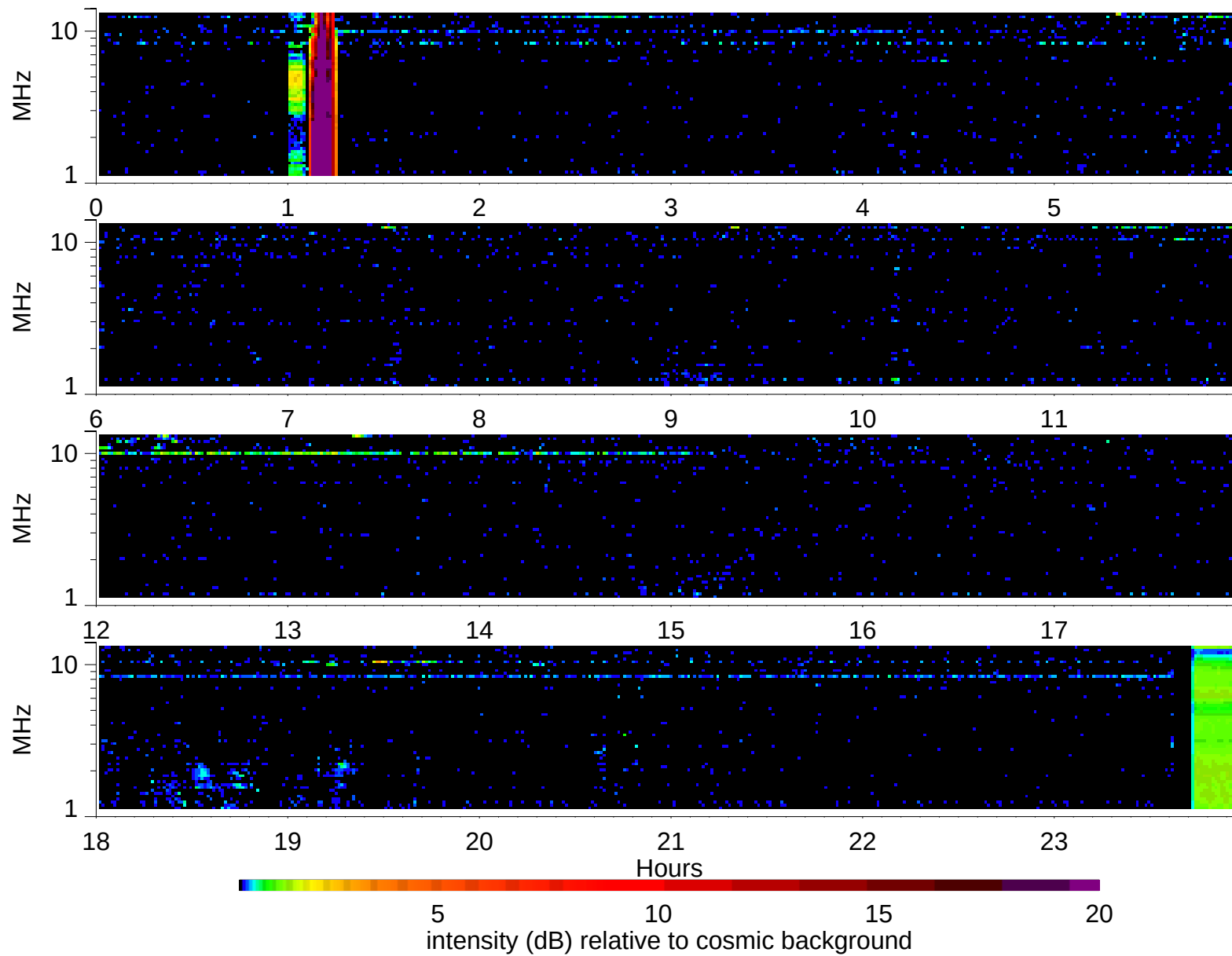
Wind Waves RAD2 receiver: 2007/10/23
