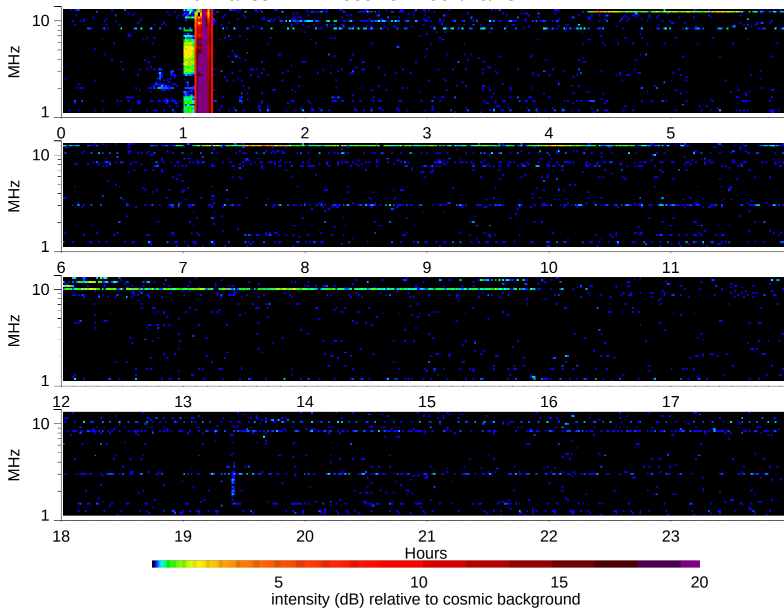
Wind Waves RAD2 receiver: 2007/10/25
