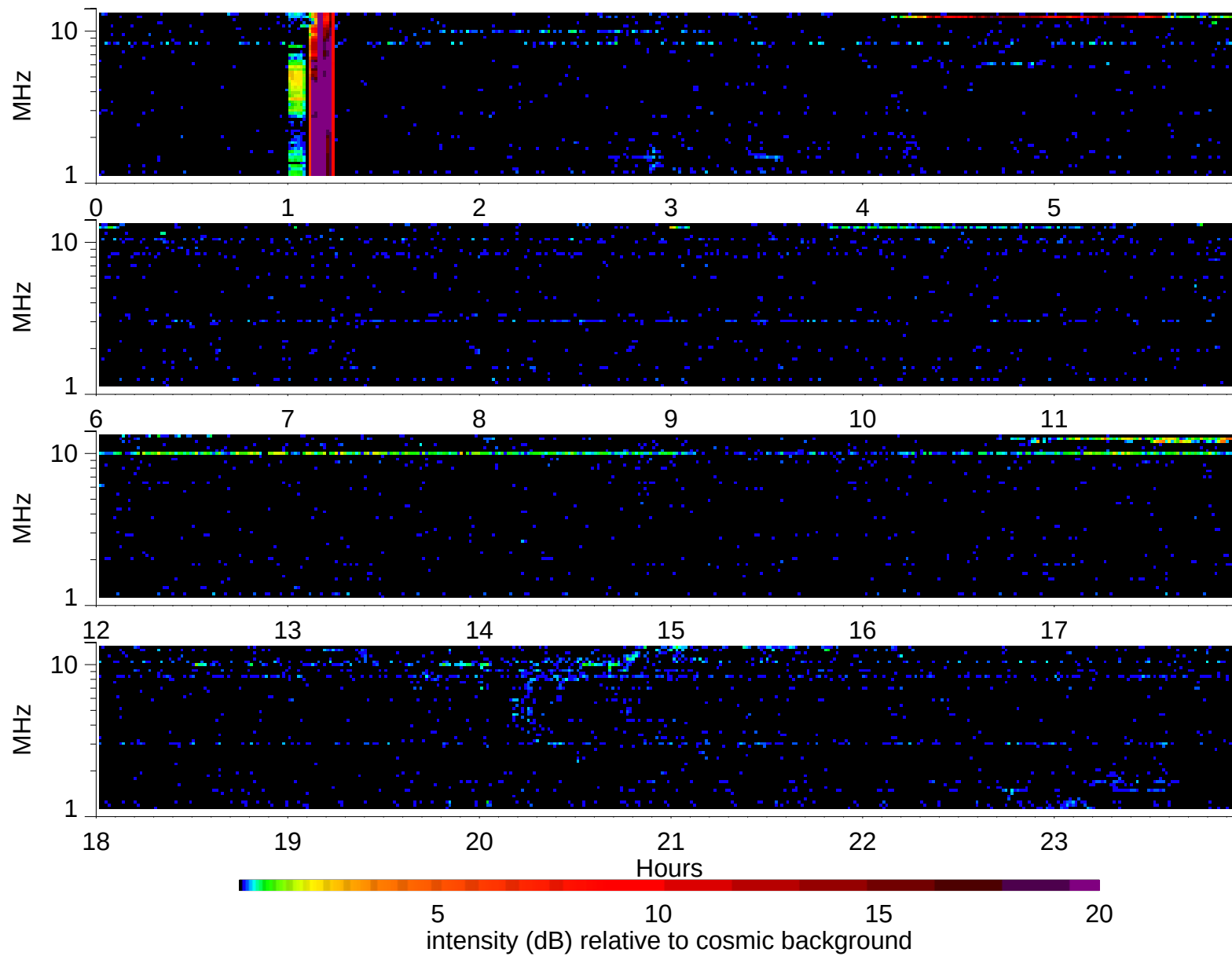
Wind Waves RAD2 receiver: 2007/11/2
