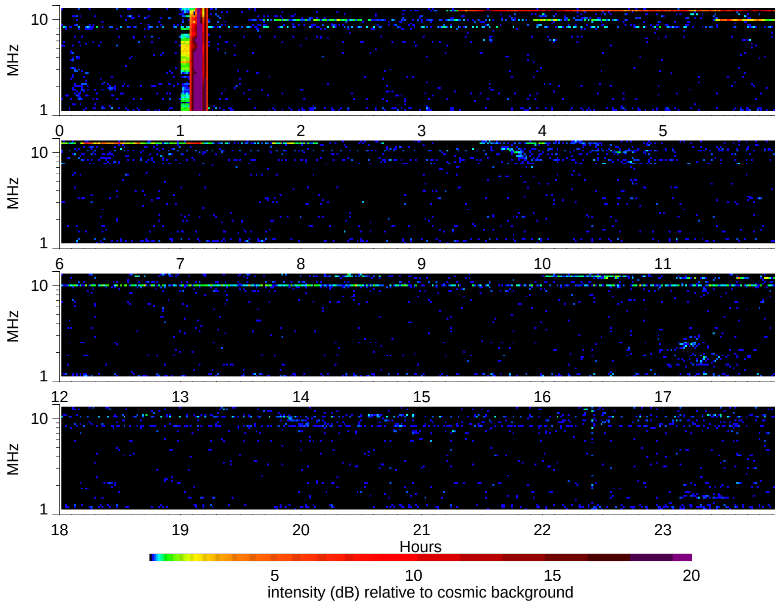
Wind Waves RAD2 receiver: 2007/11/14
