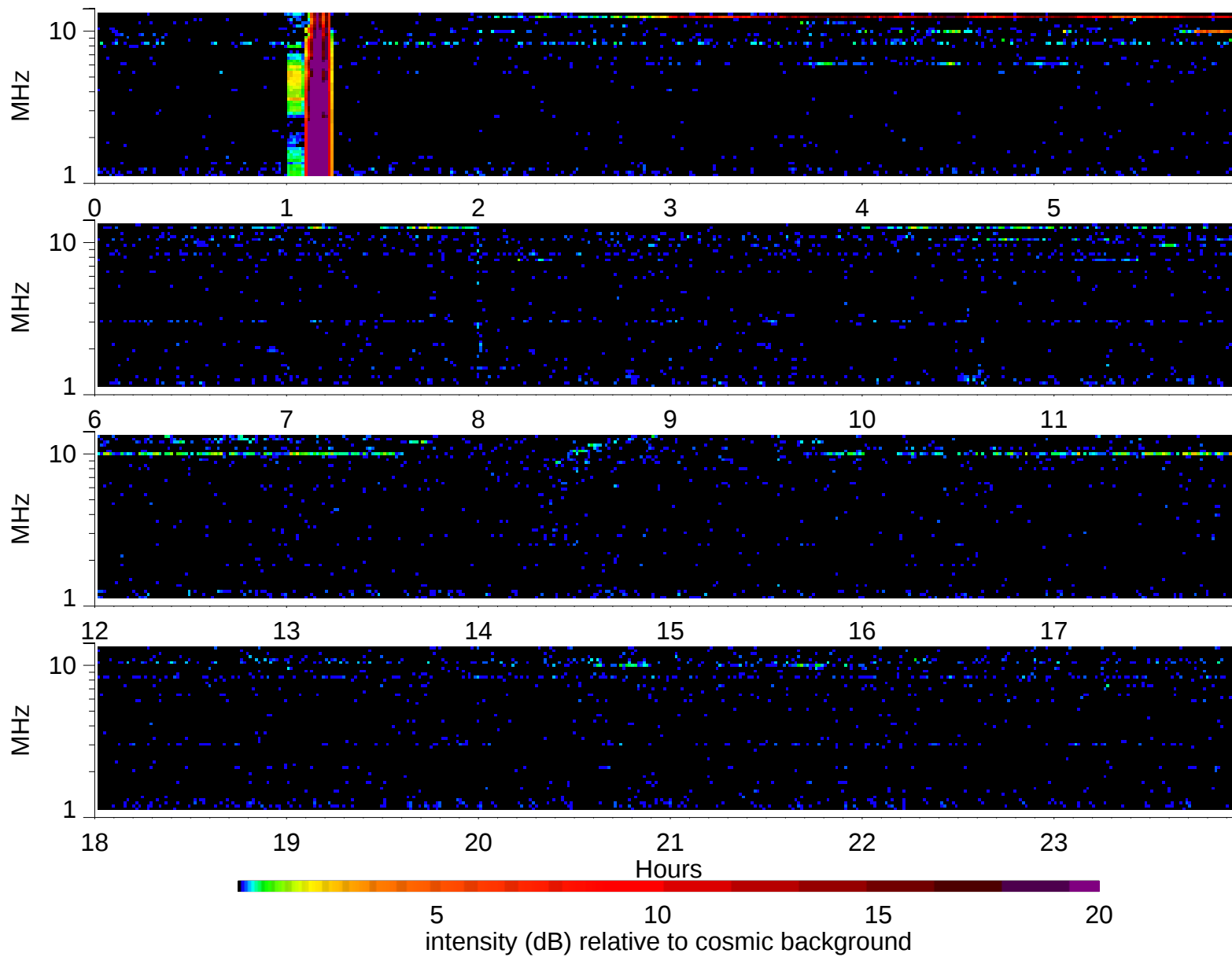
Wind Waves RAD2 receiver: 2007/11/20
