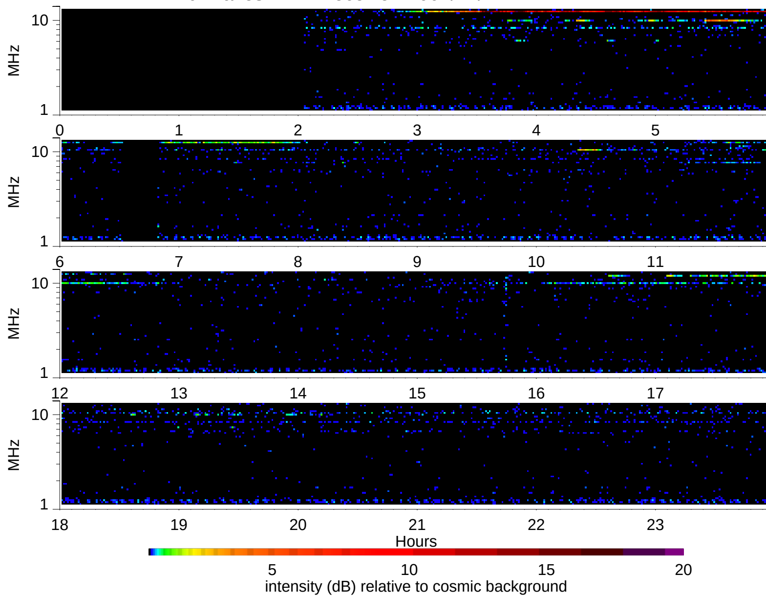
Wind Waves RAD2 receiver: 2007/11/27
