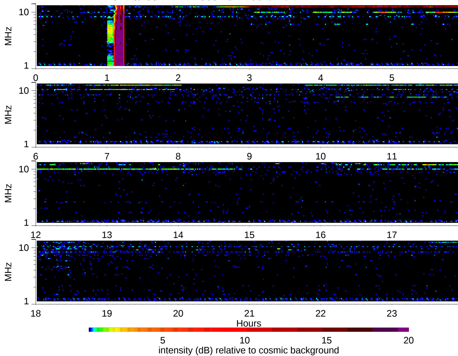
Wind Waves RAD2 receiver: 2007/12/4
