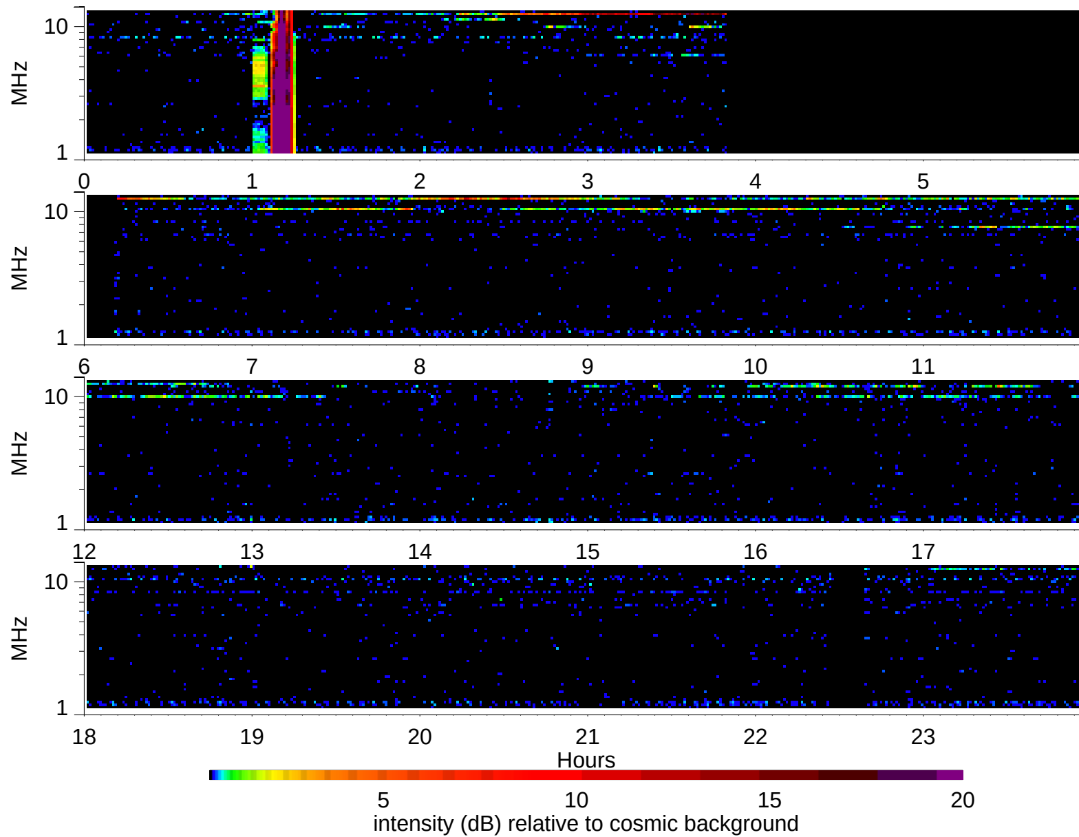
Wind Waves RAD2 receiver: 2007/12/16
