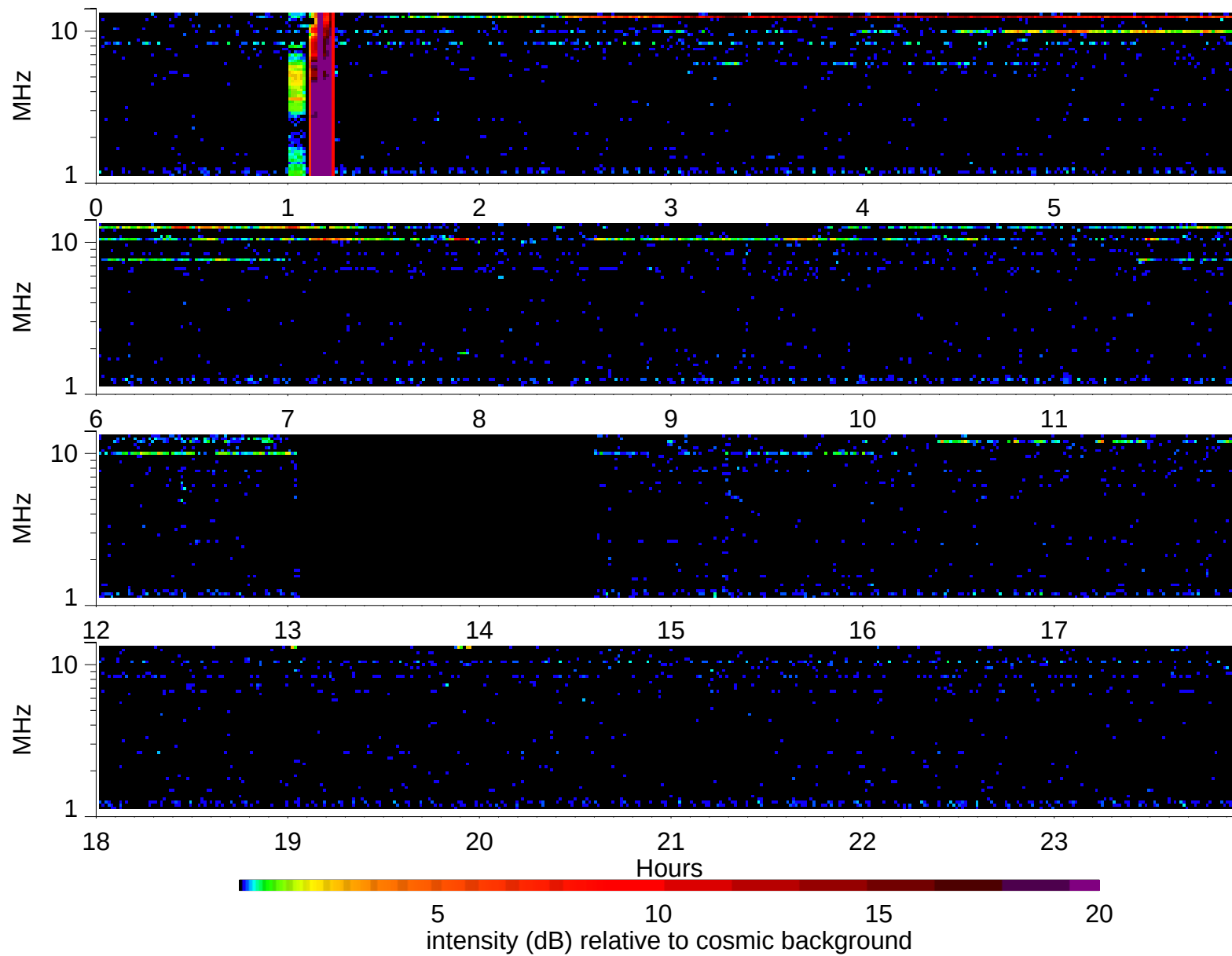
Wind Waves RAD2 receiver: 2007/12/18
