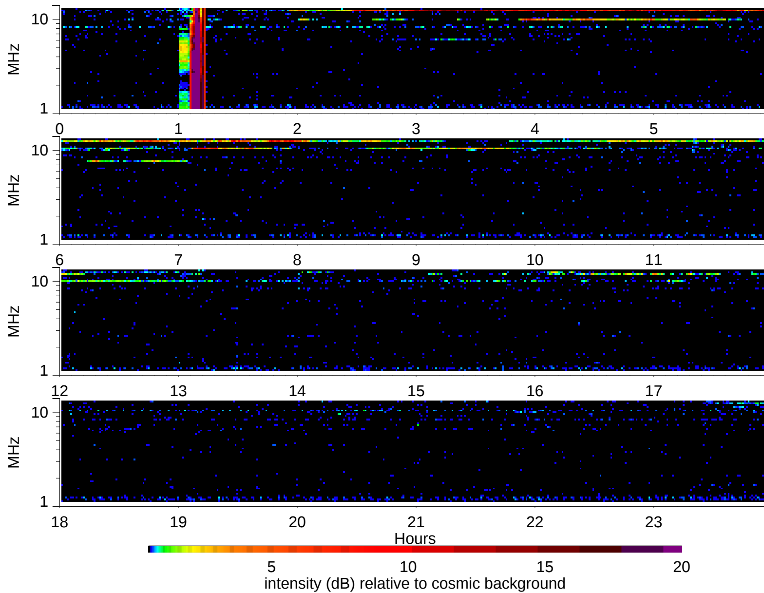
Wind Waves RAD2 receiver: 2007/12/22
