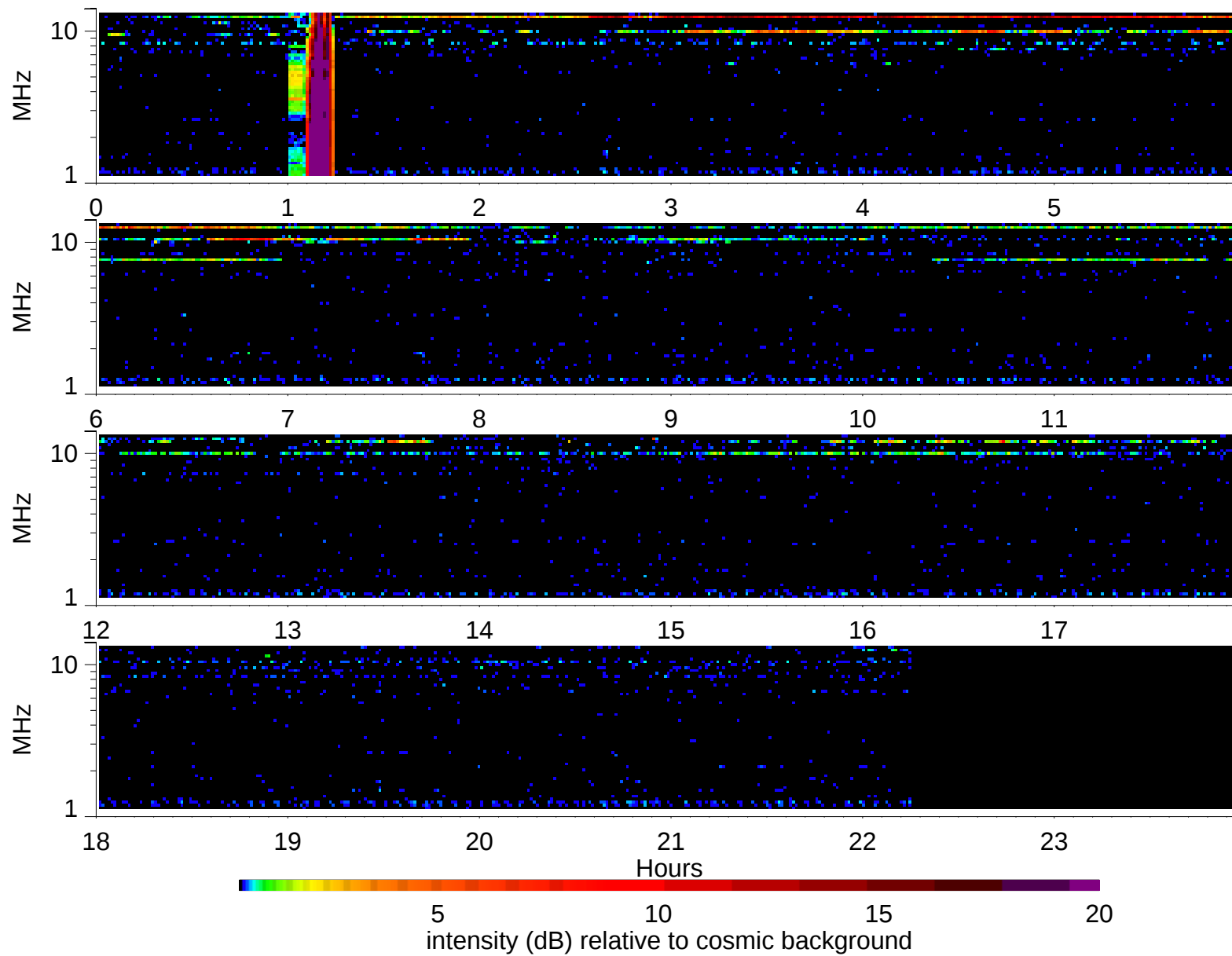
Wind Waves RAD2 receiver: 2007/12/28
