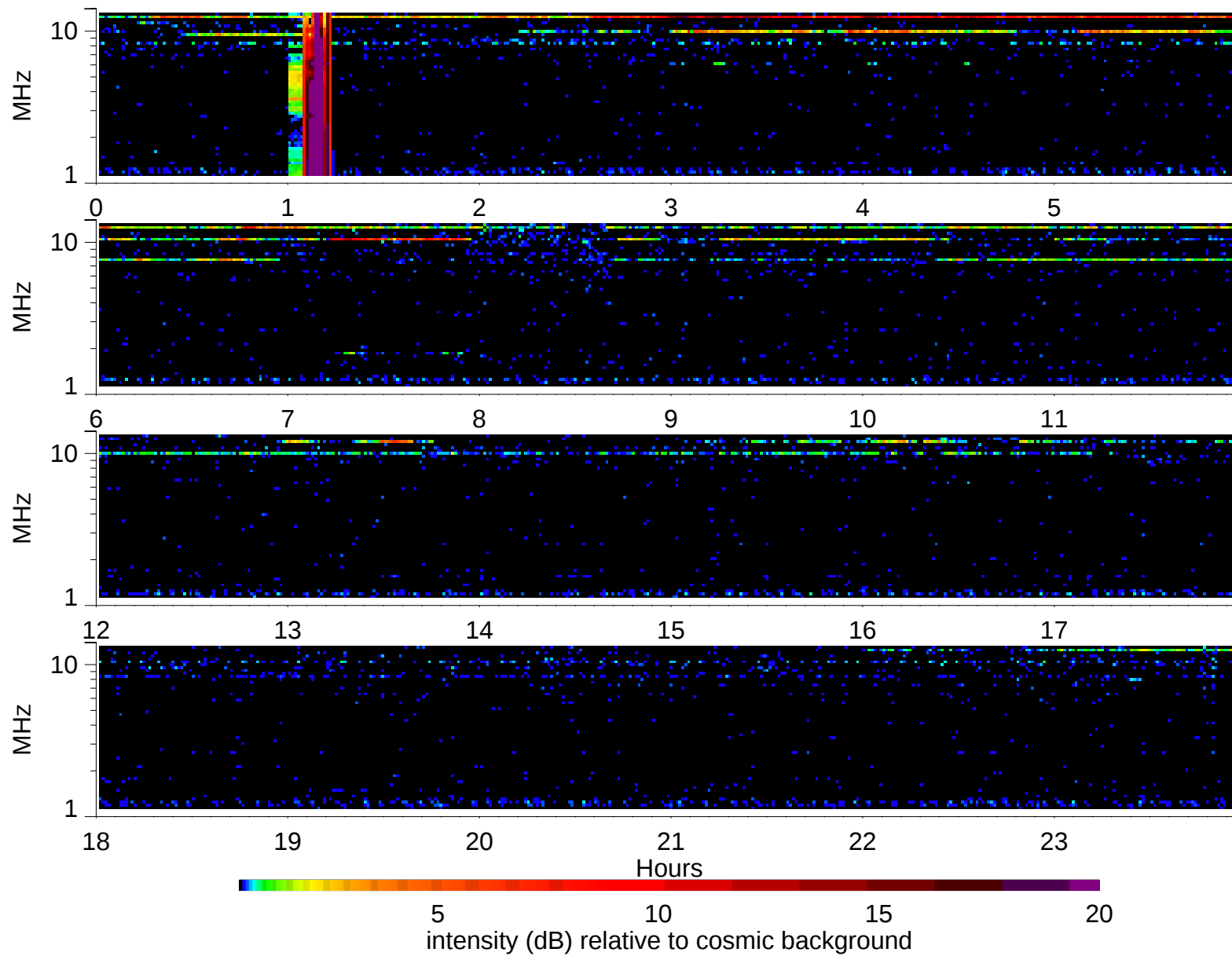
Wind Waves RAD2 receiver: 2007/12/30
