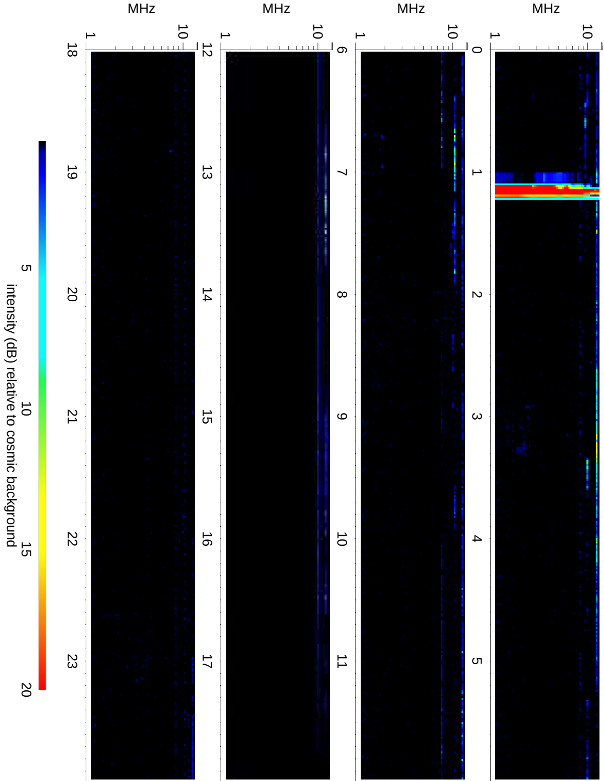
Wind Waves RAD2 receiver: 2008/01/14
