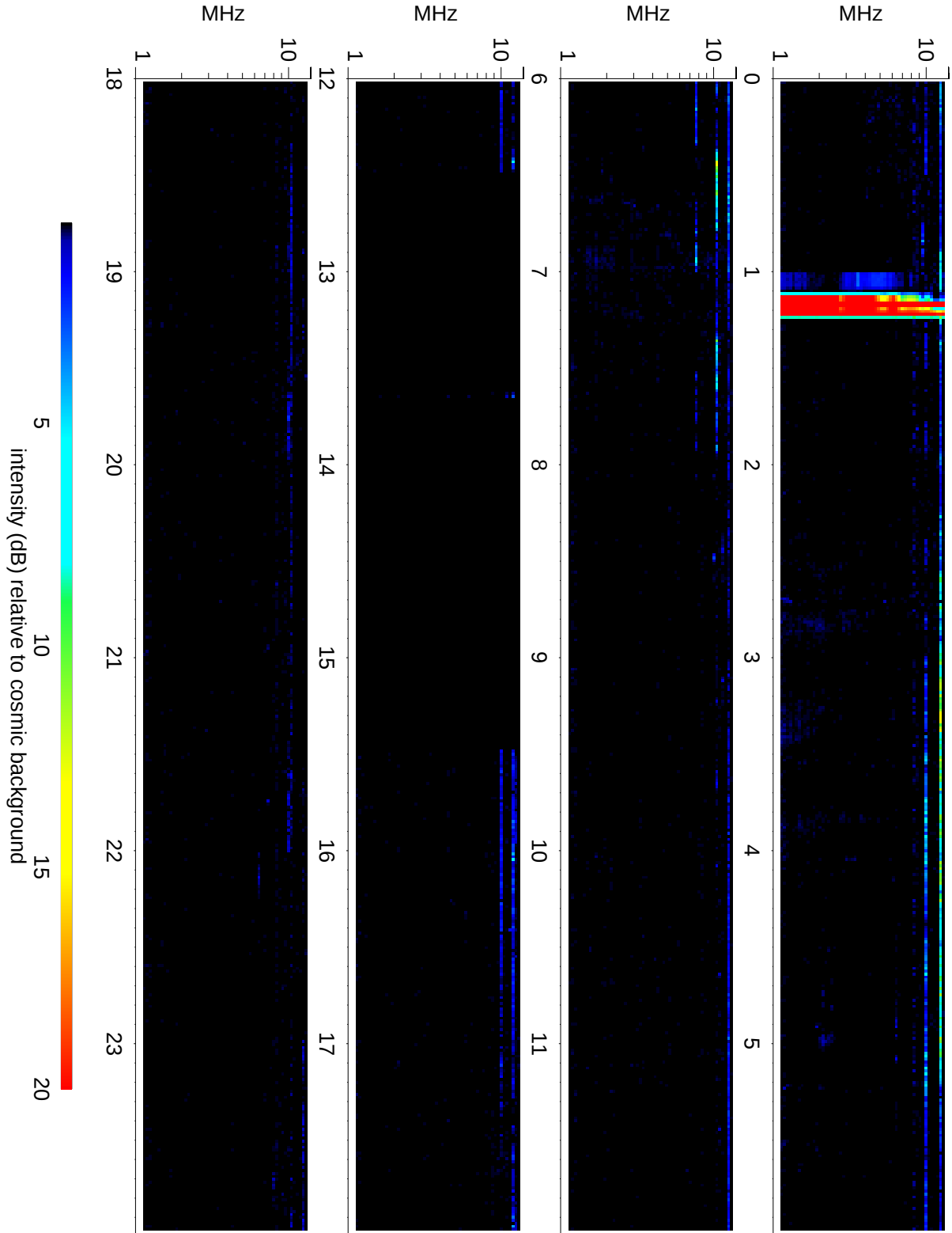
Wind Waves RAD2 receiver: 2008/01/18
