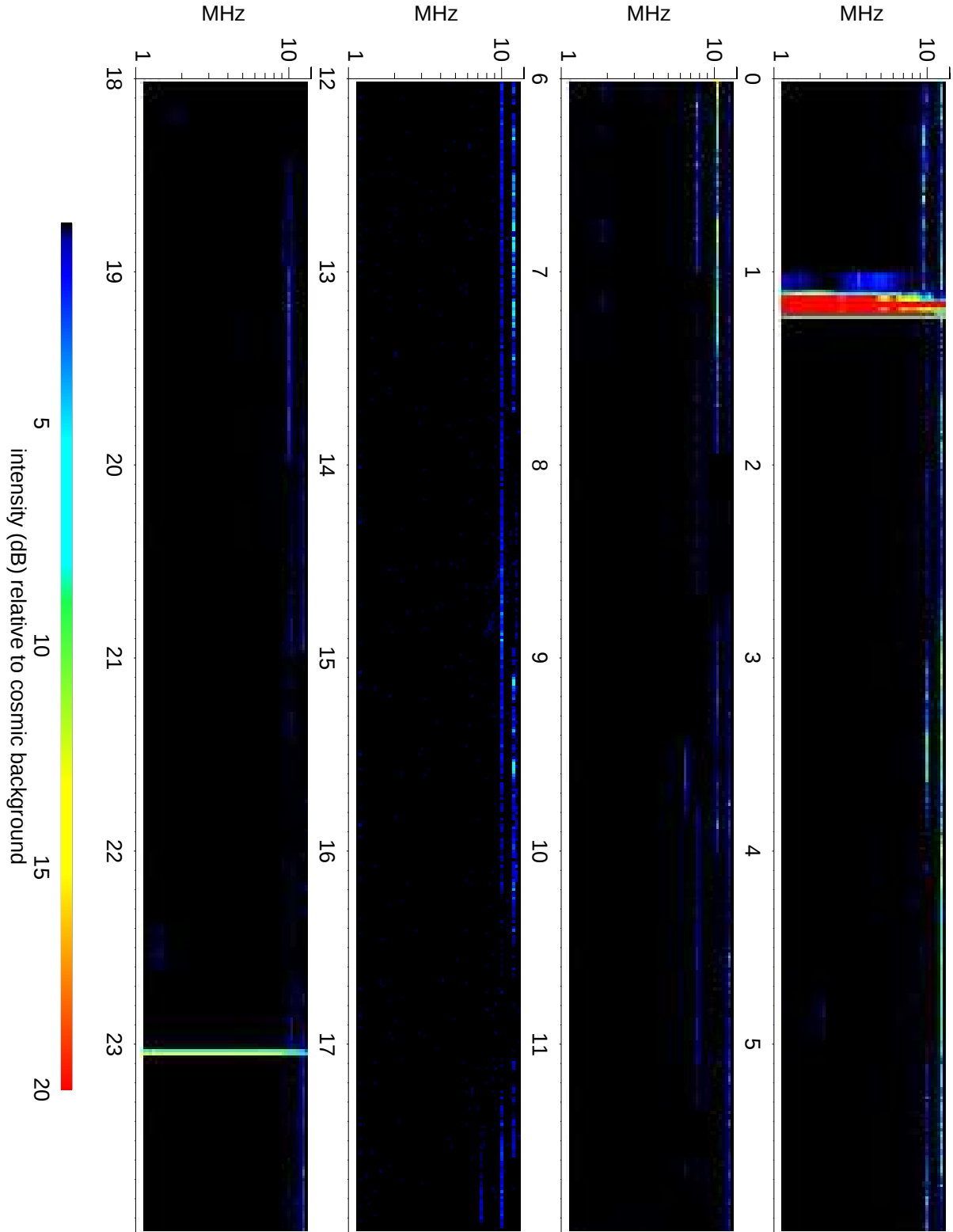
Wind Waves RAD2 receiver: 2008/01/26
